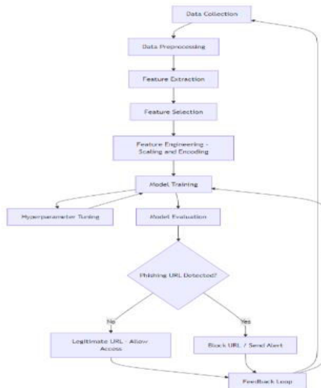
Fig 1: Flowchart of the Proposed Phishing URL Detection System
